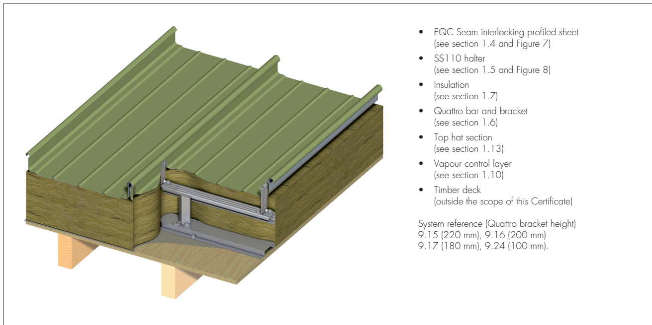
Figure 6 System 9 – on timber decking
