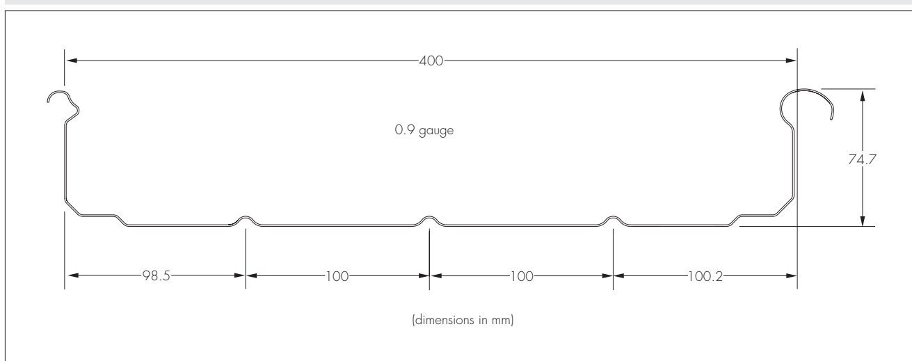
Figure 7 EQC Seam sheet profile
