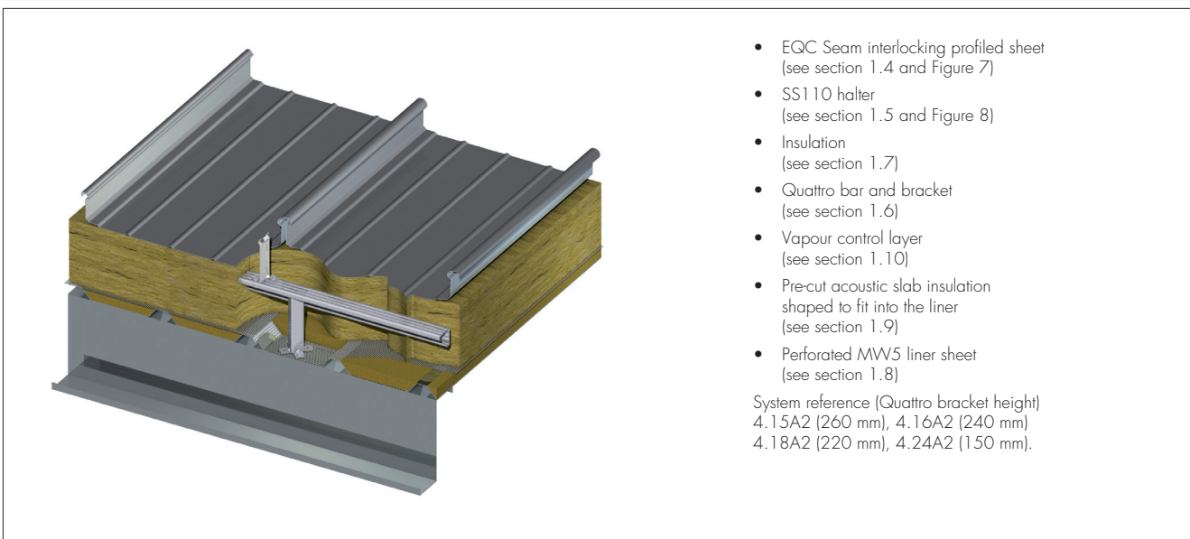
Figure 2 System 4A2 — over purlins — Acoustic Absorption System
