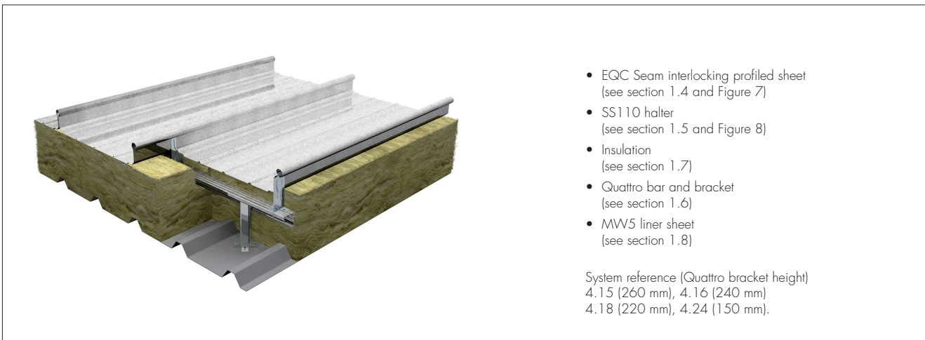
Figure 1 System 4 — over purlins — EQC Seam with Quattro bar and bracket and MW5 liner
